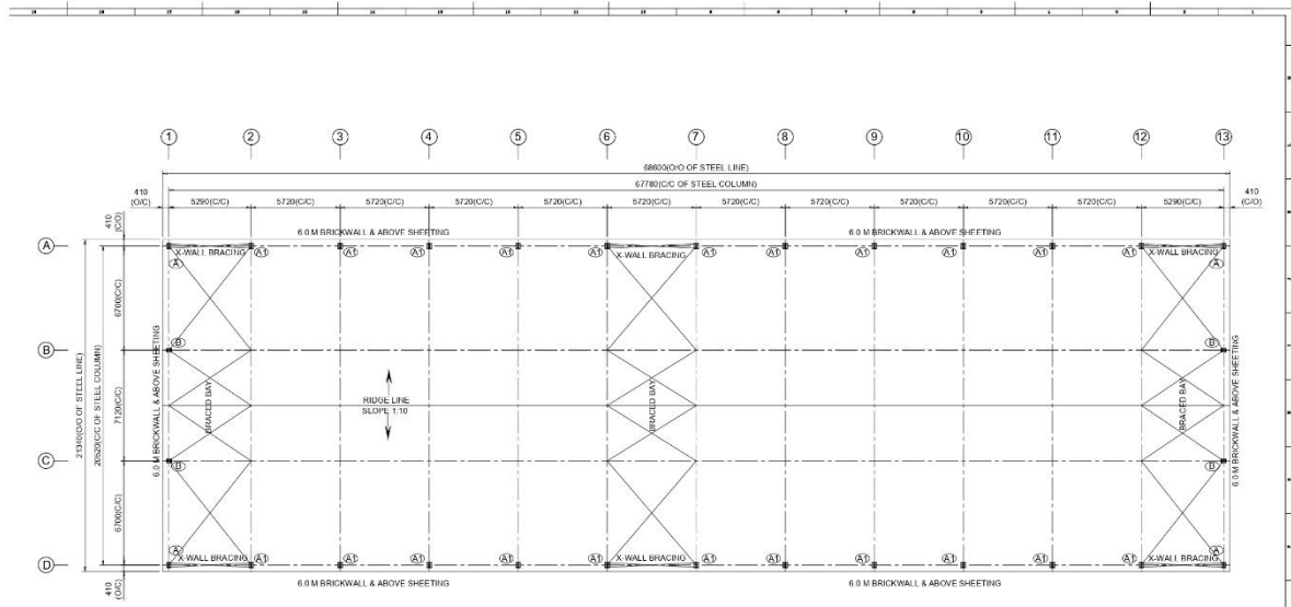
ANCHOR BOLT PLAN (NOTE: CUSTOMER TO CONFIRM ALL DIMENSIONS)
